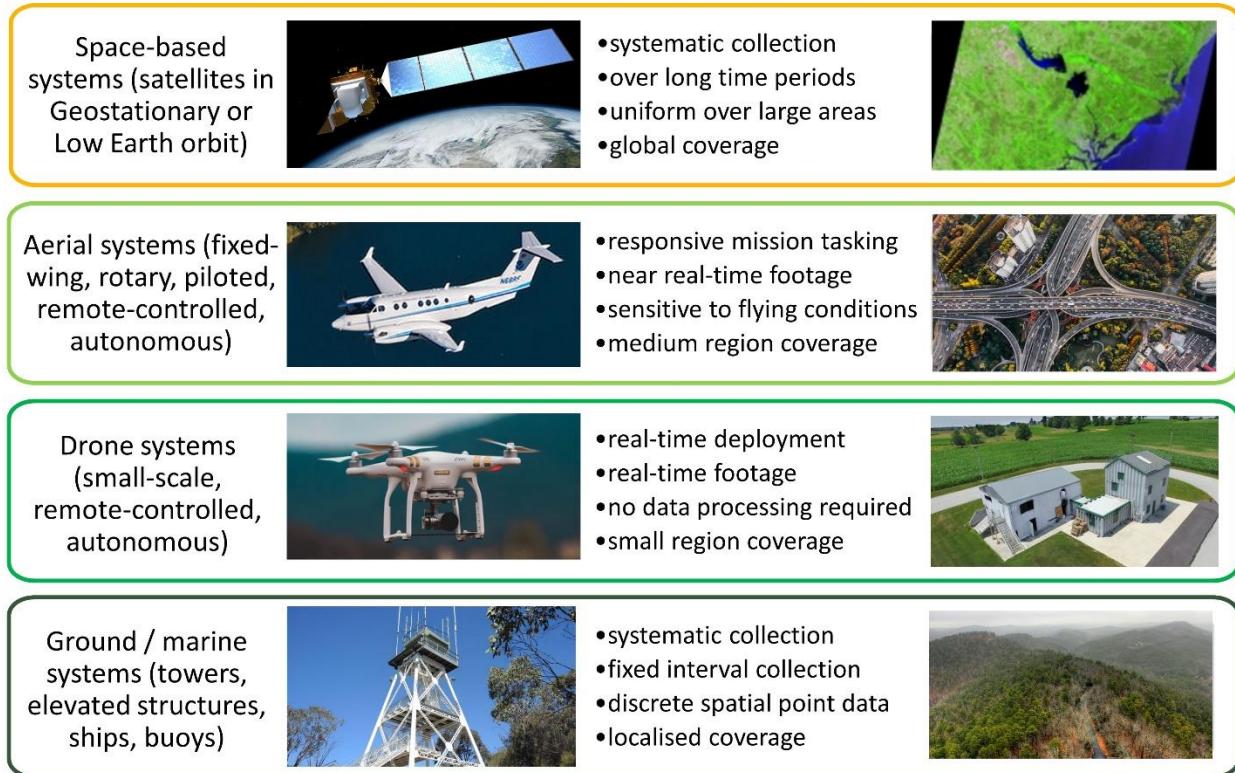
Figure 6 – Platforms for sensors
